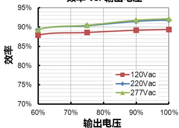
EUP-096S350ST( I_o=2625mA )
