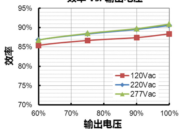
EUP-096S350ST( I_o=3500mA )
