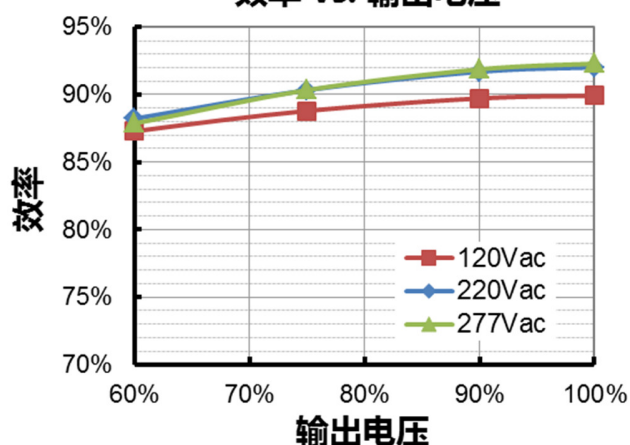
EUP-096S350ST( I_o=2625mA )
