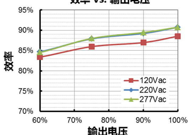
EUP-096S350ST( I_o=3500mA )
