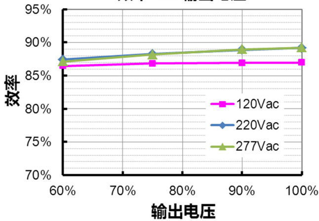
EUC-060S105DTM( I_o=1050mA )
