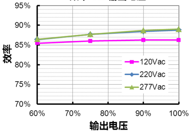
EUC-060S180DTM( I_o=1800mA )
