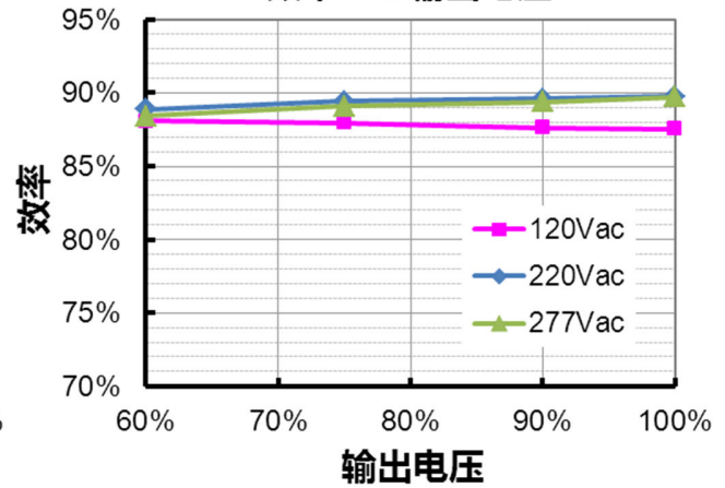
EUC-060S105DTM0004( I_o=860mA )
