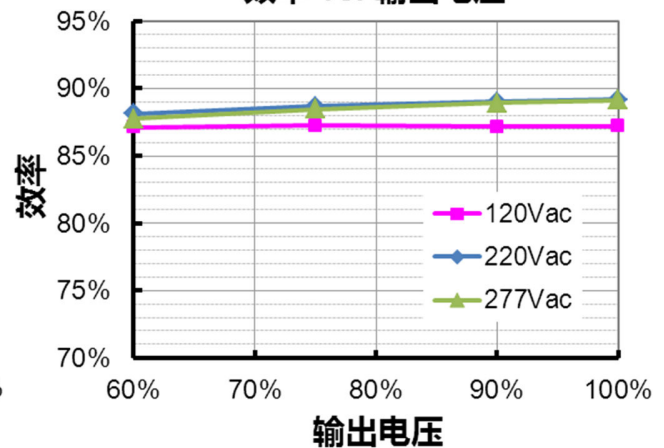
EUC-060S180DTM0004( I_o=1400mA )
