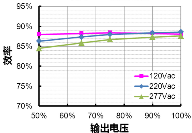
EUC-026S050SVM0003 (I o =350mA) 效率 vs. 输出电压
