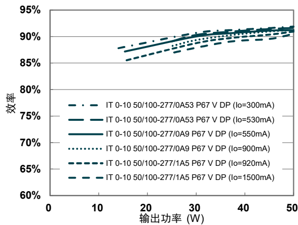
效率@230Vac
