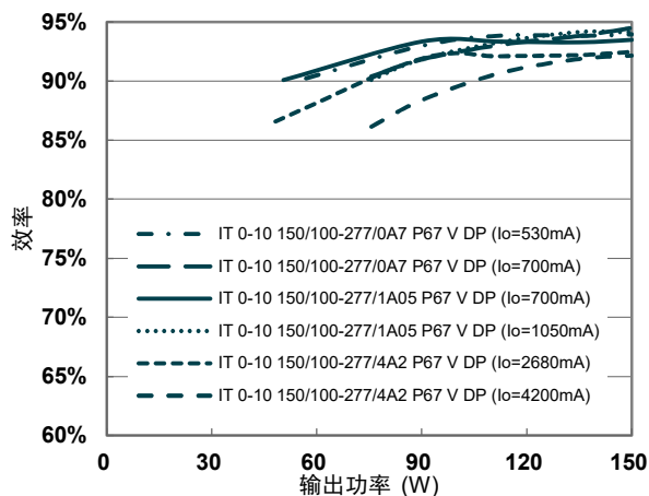
效率@230Vac
