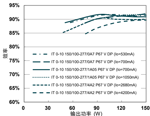
效率@230Vac
