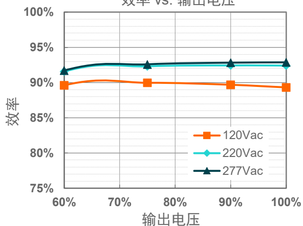
EUM-240S670Lx( I_o=4200\text{mA} )
