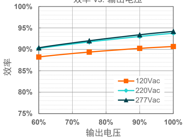
EUM-240S350Lx( I_o=3500\text{mA} )
