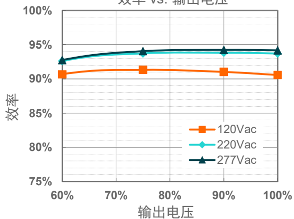
EUM-240S350Lx( I_o=2150\text{mA} )
