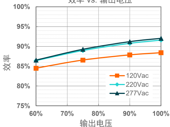
EUM-240S670Lx( I_o=6700\text{mA} )
