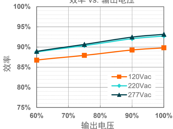
EUM-240S670Lx( I_o=6700\text{mA} )
