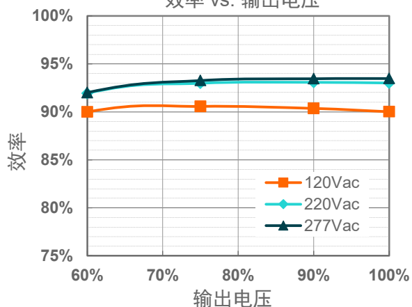
EUM-240S670Lx( I_o=4200\text{mA} )
