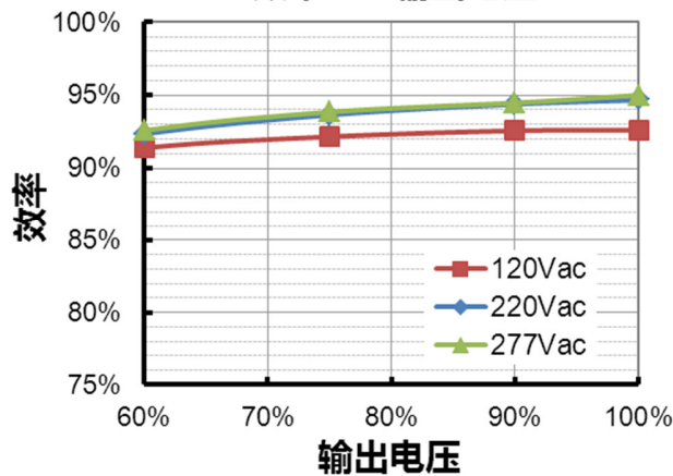
EUD-600S420DV( I_o=3360mA ) 效率 vs. 输出电压
