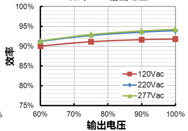
EUD-600S420DV( I_o=4200mA ) 效率 vs. 输出电压
