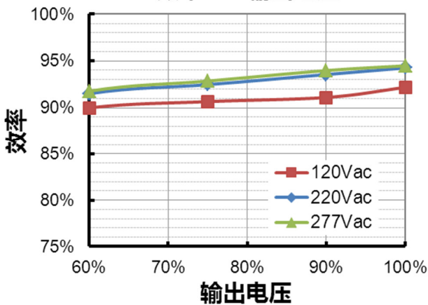
EUD-600S980DV (Io=7840mA) 效率 vs. 输出电压
