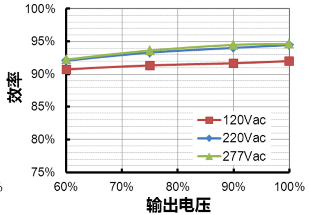
EUD-600S280DV( I_o=2800mA ) 效率 vs. 输出电压
