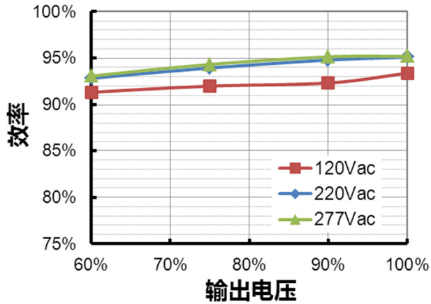
EUD-600S280DV( I_o=2240mA ) 效率 vs. 输出电压
