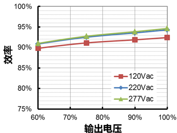
EUM-320S150Lx( I_o=1500mA ) 效率 vs. 输出电压
