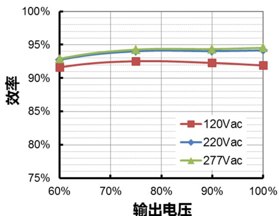
EUM-320S250Lx( I_o=1750mA ) 效率 vs. 输出电压
