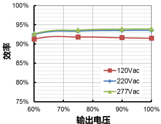
EUM-320S500Lx( I_o=2850mA ) 效率 vs. 输出电压
