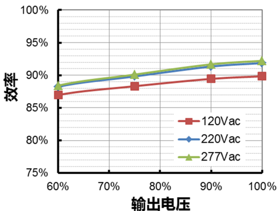
EUM-320S760Lx( I_o=7600mA ) 效率 vs. 输出电压
