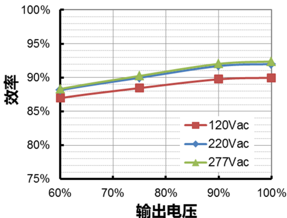
EUM-320S500Lx( I_o=5000mA ) 效率 vs. 输出电压
