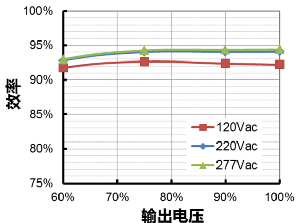
EUM-320S150Lx( I_o=1050mA ) 效率 vs. 输出电压
