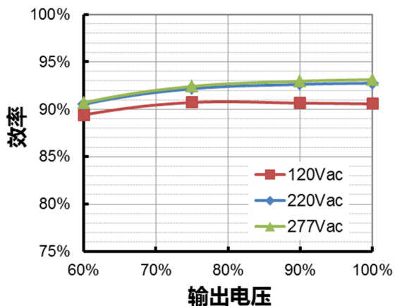
EUM-320S760Lx( I_o=5350mA ) 效率 vs. 输出电压
