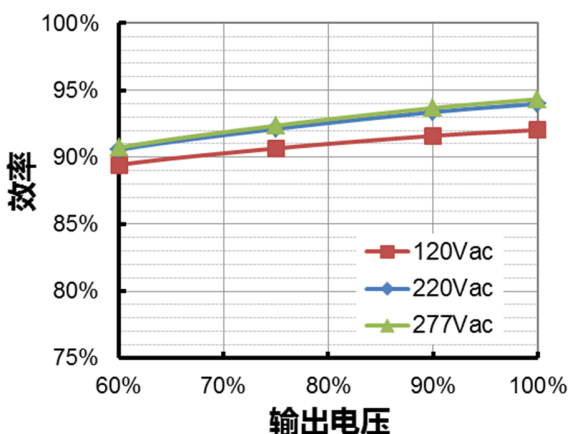
EUM-320S250Lx( I_o=2500mA ) 效率 vs. 输出电压
